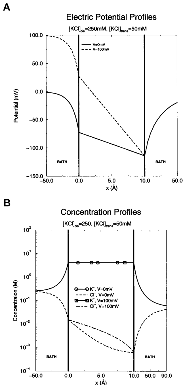
FIGURE 4 (A) Profile of the potential in asymmetrical 250 || 50 mM solutions. Note the large region in which the potential in the baths differs from its bulk value (for this reason the scale of the horizontal axis is different inside the channel, 0 < x < 10 Å, and outside the channel in the baths, x < 0 and x > 10 Å). The potential profiles are clearly sensitive functions of transmembrane potential and bath concentration. (B) Profile of the concentration of anions and cations in asymmetrical 250 || 50 mM solutions with a logarithmic vertical axis and different horizontal scales inside and outside the channel. The forward and backward rate constants for the permeation of each ion are determined by the potential profiles as shown in the Appendix, Eqs. 2–4. The dependence is considerable, as documented in Table 3. Roughly speaking, in this channel, changing one solution from 250 mM to 50 mM changes the rate constants by a factor of 2–10; changing the transmembrane potential by 100 mV changes the forward and backward rate constants by a factor of 10.
