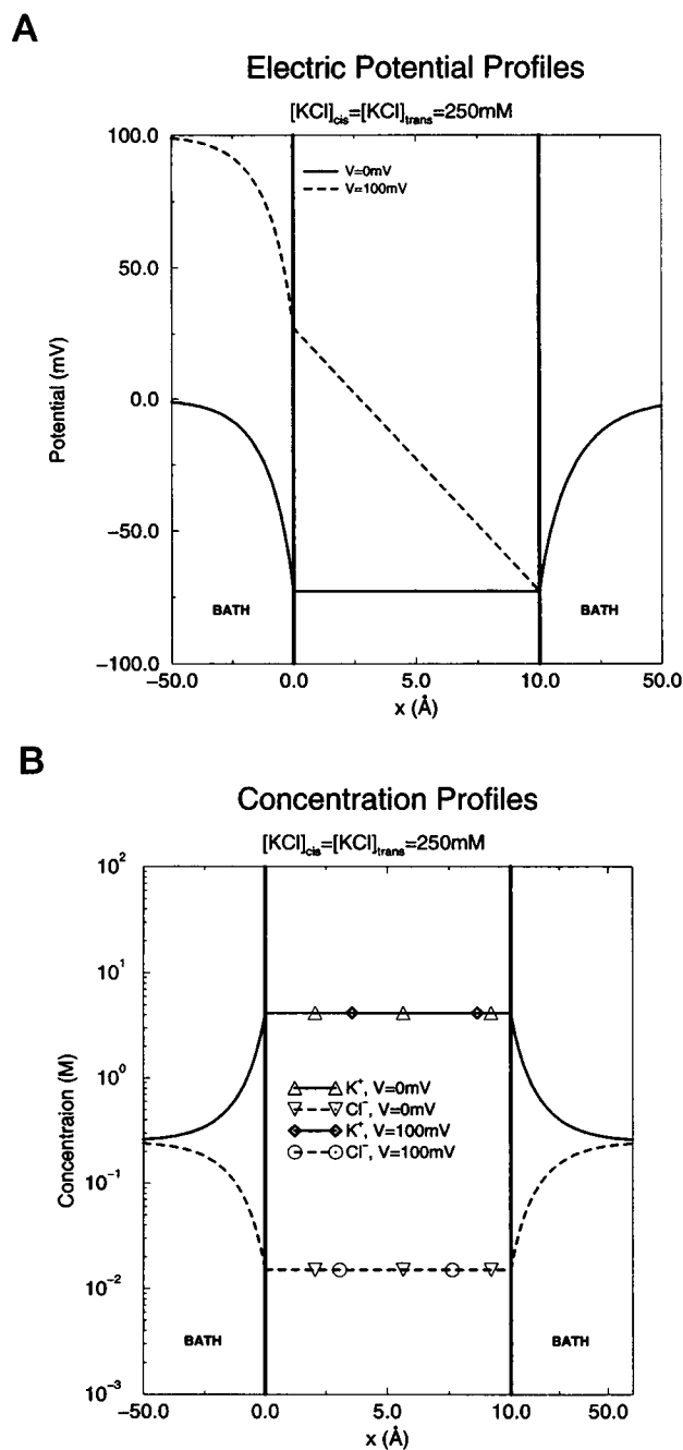
FIGURE 3 (A) Profile of the potential in symmetrical 250 mM solutions. Note the large region in which the potential in the baths differs from its bulk value (for this reason the scale of the horizontal axis is different inside the channel, 0 < x < 10 Å, and outside the channel in the baths, x < 0 and x > 10 Å). This region is so large because the concentration of permanent charge at the ends of the channel is so large (see Fig. 1) compared to the concentration of the bathing solutions. The Debye length in the channel is thus much shorter than the Debye length in the bath. The potential profiles are clearly sensitive functions of transmembrane potential and bath concentration. See caption of Fig. 4. (B) Profile of the concentration of anions and cations in symmetrical 250 mM solutions with a logarithmic vertical axis and different horizontal scales inside and outside the channel. The concentration profiles show much less dependence on transmembrane potential and bath concentration than the potential profiles. This is to be expected from a channel like CRC with (nearly) linear I - V relations, and is not found in channels with more complex profiles of fixed charge and thus more complex I - V characteristics (Chen et al., 1995b, 1997; Tang et al., 1997).
